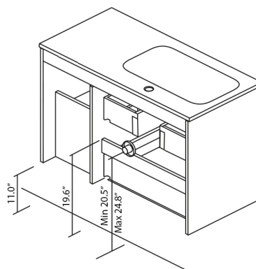
2 Drawers - 1 Door
